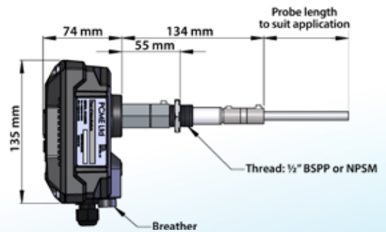
Standard Sensor 125°C
