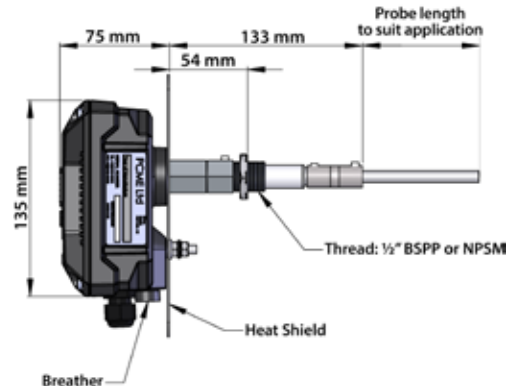
Standard Sensor 125°C
