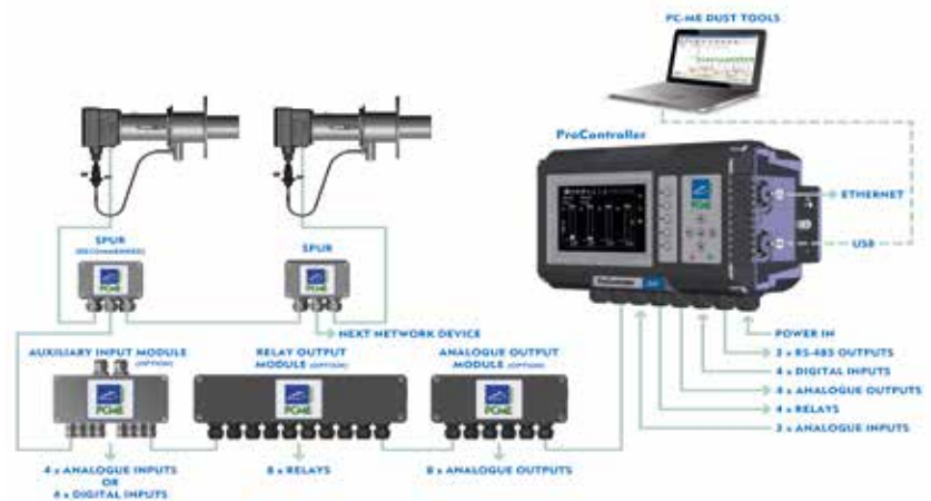
QAL 360s sensors used in a network system
